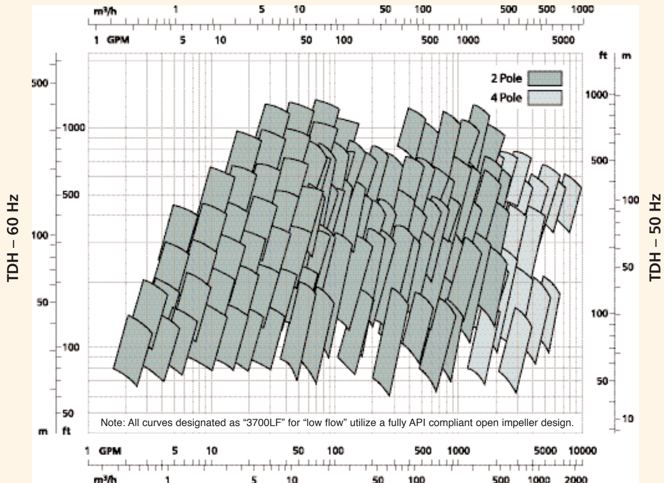
Flow Rate – 60 Hz
